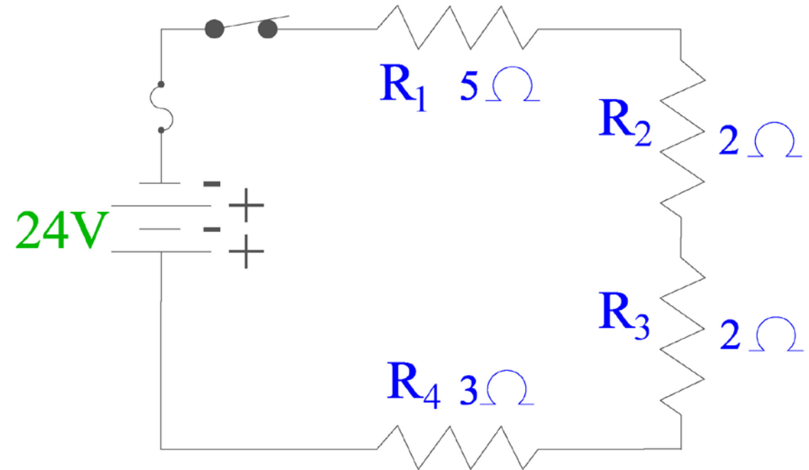
Series Connection
