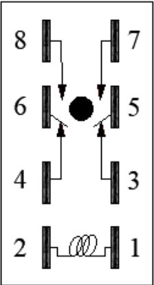
Socket View
