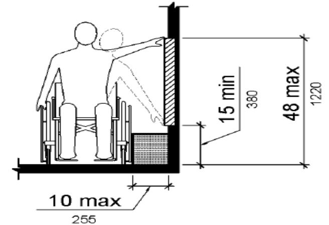
Figure 308.3.1 Unobstructed Side Reach
