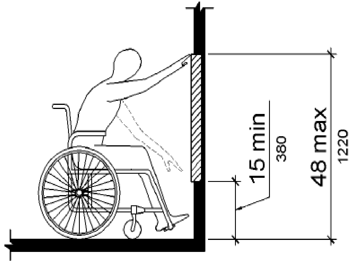
Figure 308.2.1 Unobstructed Forward Reach
