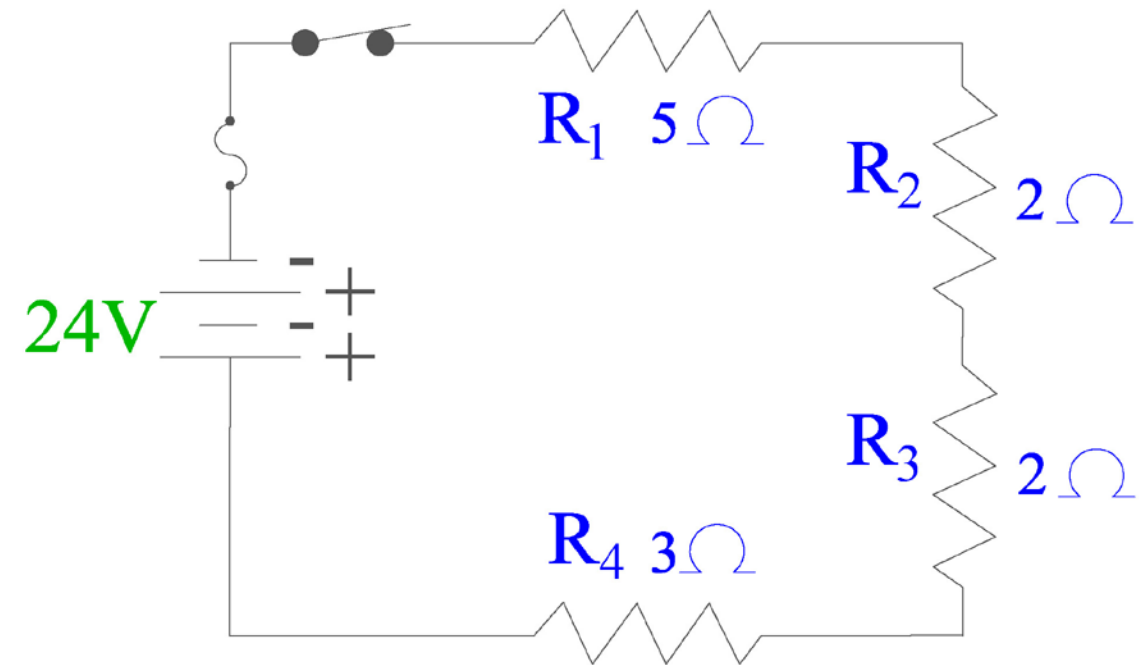
Series Connection
