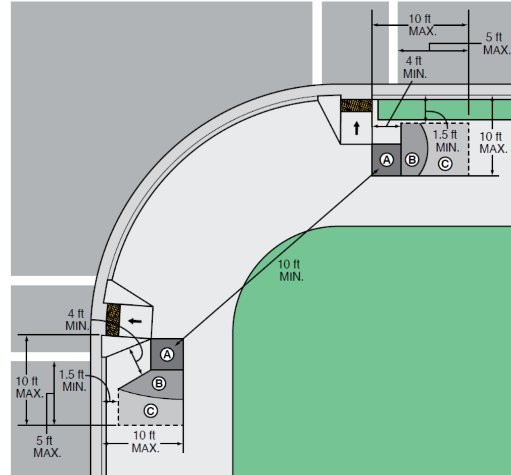
Figure 4I-2. Preferred Push Button Location Area
