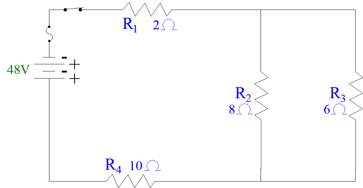
Series/Parallel Connection
